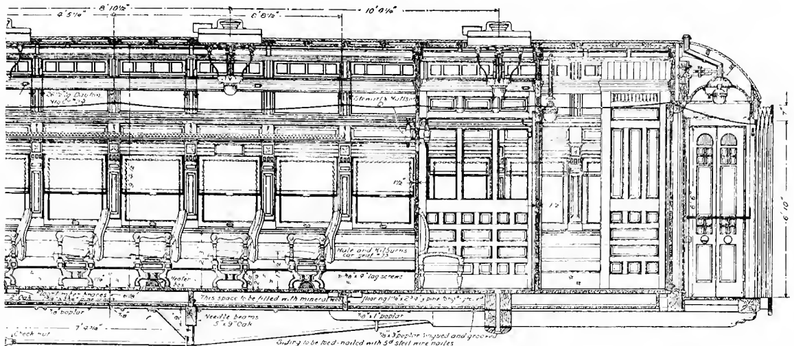
Fig. 422. Half Side Elevation of Interior.
